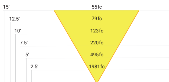
340 WATT - Forward Throw
