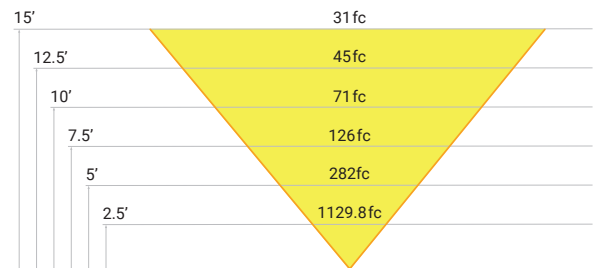
200 WATT - Wide Forward Throw
