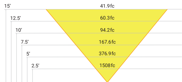
270 WATT - Wide Forward Throw
