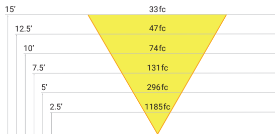
200 WATT - Forward Throw
