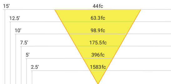
270 WATT - Forward Throw
